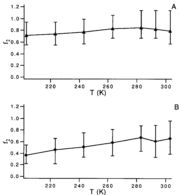
FIGURE 12 Fractional population ( f_2 ) of transferring molecules on edge excitation. (A) Data for LipDH-AV. (B) Data for LipDH-Δ14.
