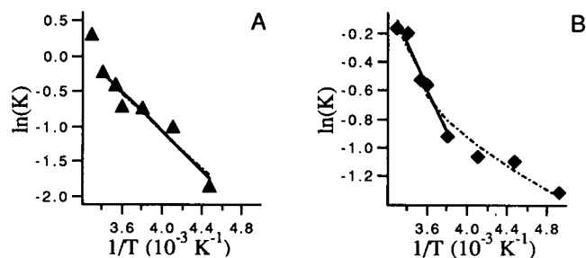
FIGURE 4 van 't Hoff plot of equilibrium constants of conformational transition. (A) Data for LipDH-AV. (B) Data for LipDH-Δ14. (—) Linear fit to experimental data.
