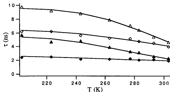
FIGURE 3 Temperature dependence of barycenters of the lifetime distributions. (▲) LipDH-AV, (◆) LipDH-Δ14, (△, ◇) Longest lifetime class, (▲, ◆) Shortest lifetime class, (—) Best fit of data to Eq. 8.
